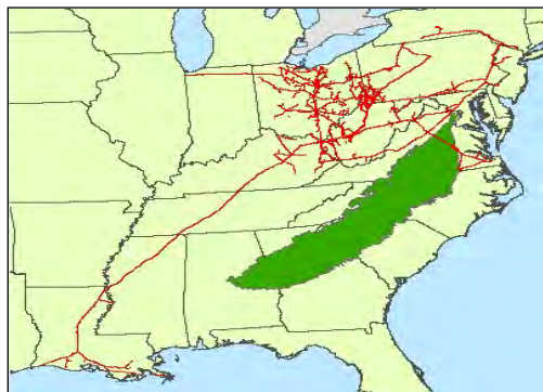
Figure 3.3-17: Piedmont Ecoregion
