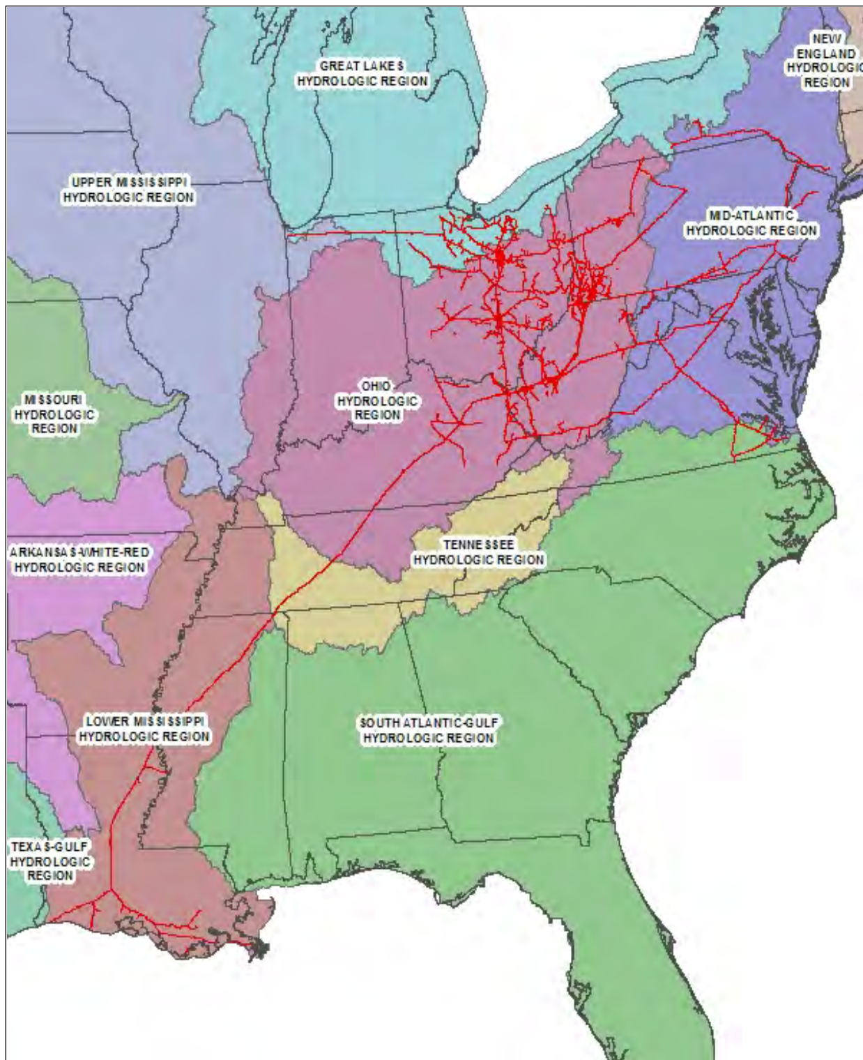
Figure 3.2-1: Hydrological Units
